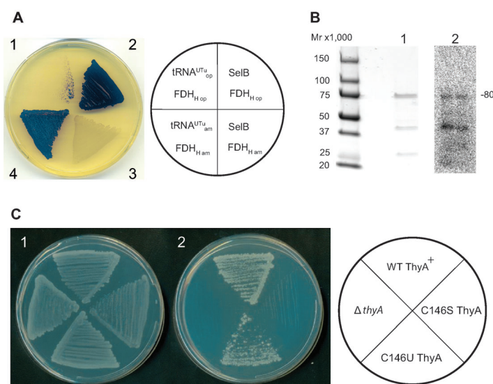
Figure 2. A) tRNA UTu mediates functional Sec incorporation in FDH H . An E. coli \Delta selA , \Delta selB , \Delta fdhF deletion strain was complemented with E. coli Sela, M. jannaschii PSTK, and 1) tRNA UTu op and FDH Hop ; 4) tRNA UTu am and FDH Ham . Controls lacked 2) tRNA UTu op or 3) tRNA UTu am , and tested FDH Hop and FDH Ham with genomic E. coli tRNA Sec and recombinant SelB. FDH H activity was visualized by the purple color in a benzyl viologen assay. B) 75 Se incorporation into E. coli FDH H . The E. coli culture described in (A4) was grown in the presence of [ 75 Se]selenite. 6xHis-tagged FDH H protein was purified and analyzed by SDS-PAGE (lane 1) followed by autoradiography (lane 2); FDH H corresponds to the protein band of approximately 80 kDa. C) ThyA C146U restores thymine prototrophy. An E. coli \Delta selA , \Delta selB , \Delta thyA deletion strain was complemented with wild-type thyA + , thyA 146Ser or thyA 146am plasmids along with tRNA UTu am and Sela. All clones showed growth on M9 minimal medium supplemented with thymine (1) while only thyA 146am (expressing C146U ThyA) was able to reconstitute the wild-type phenotype (ThyA + ) on M9 minimal medium in the absence of thymine (2).
